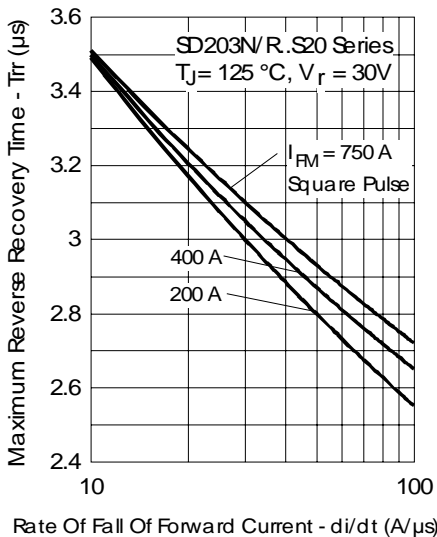
Fig.16 - Recovery Time Characteristics
