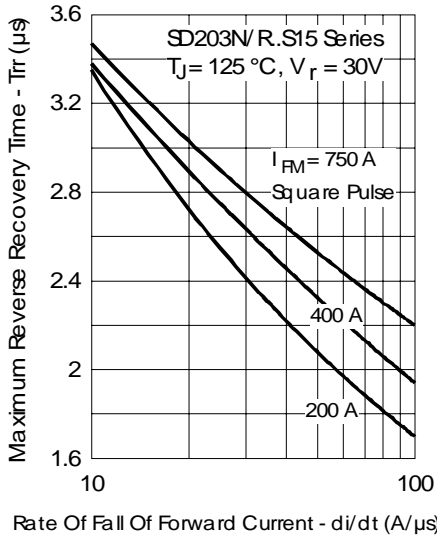
Fig.13 - Recovery Time Characteristics
